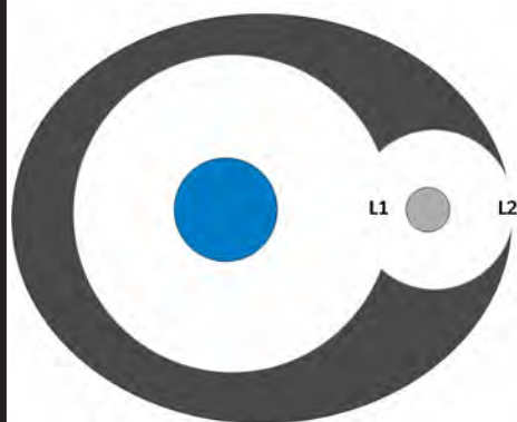
Figure 9 showing Lagrange points L1 and L2
